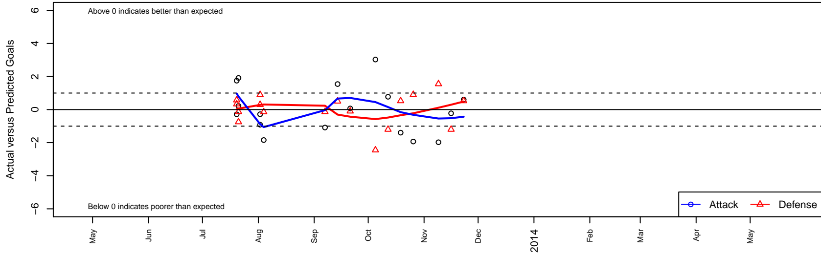
Stingrays G99 Dots are actual minus expected GF (blue circles) and GA (red triangles). Blue line is smoothed change in attack strength. Red is smoothed change in defense strength.
